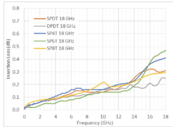
Typical Performance: DC to 18 GHz Switches
