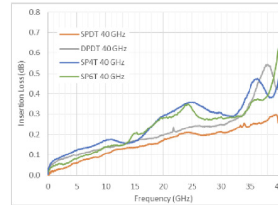
Typical Performance: DC to 40 GHz Switches
