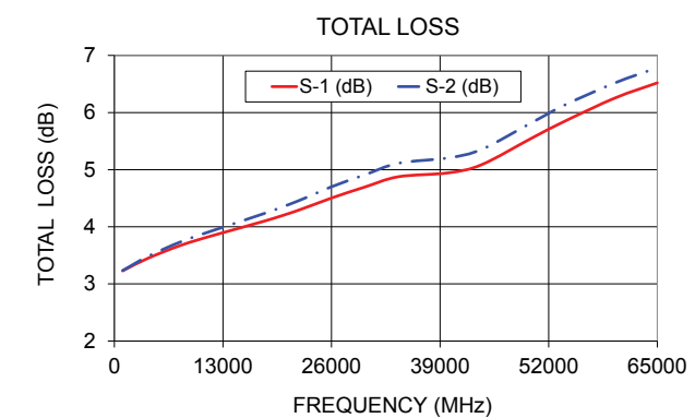
ZC2PD-E1653+ Curves
