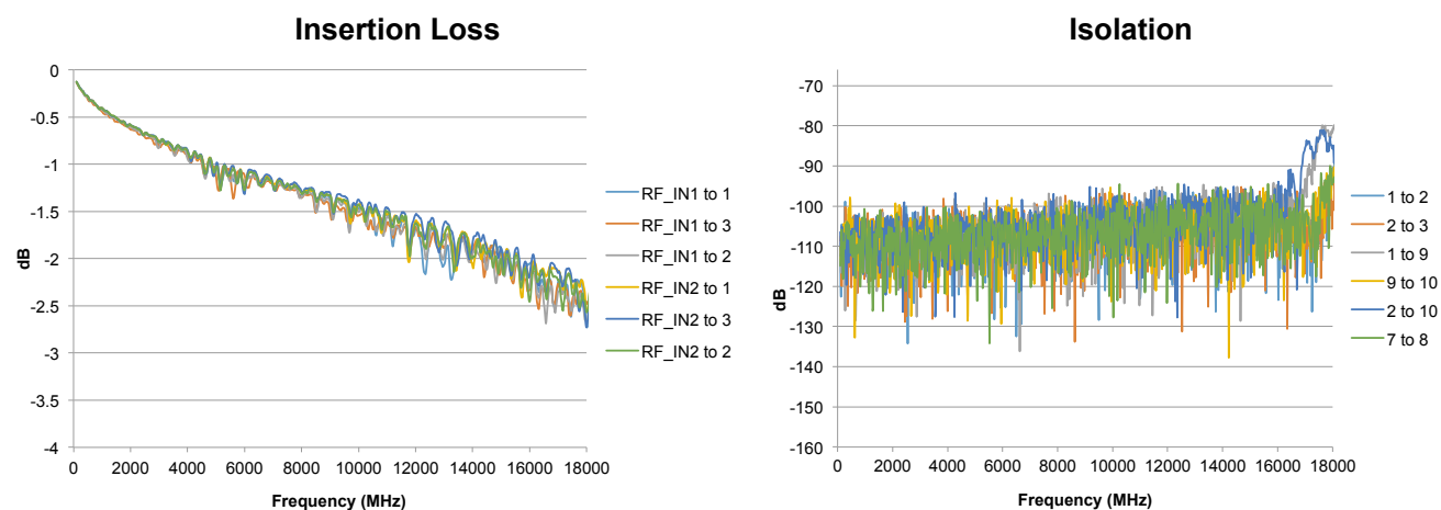
ZT-180 Curves
