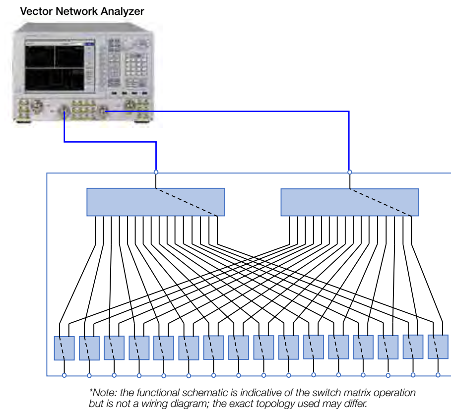
ZT-180 Functional Schematic
