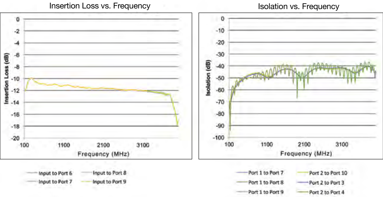
ZT-10HPS-272 Curves
