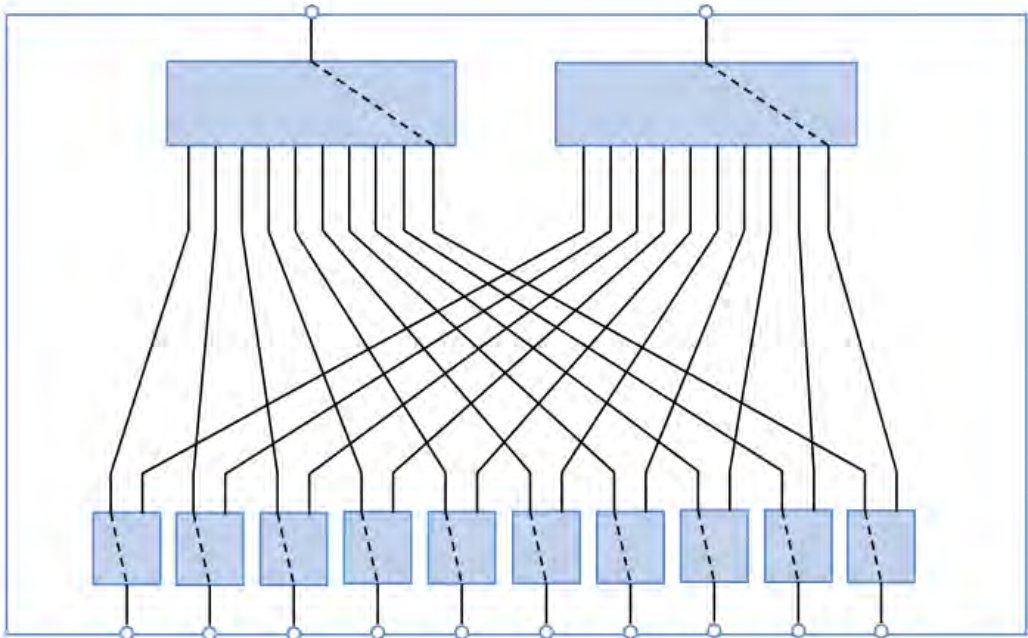
Functional schematic for ZT-209
