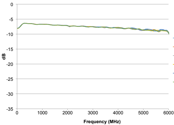
Typical Path Loss
