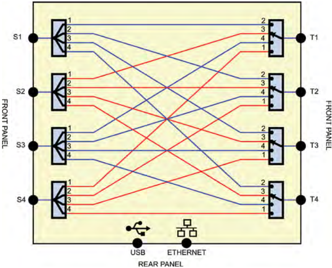
Functional Schematic
