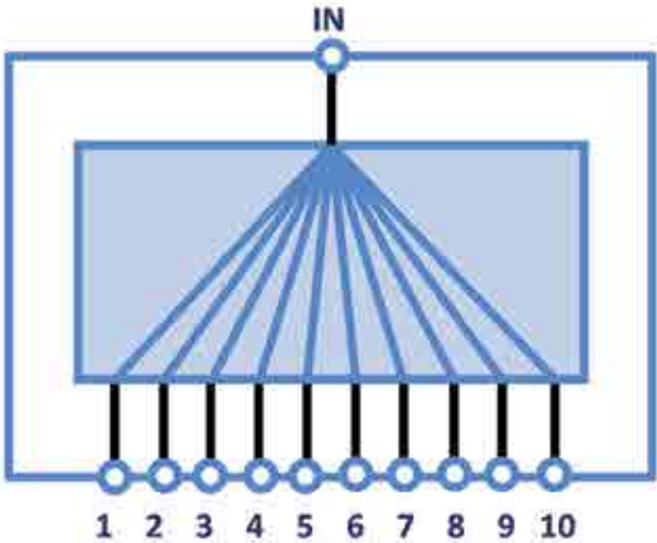
Functional Schematic
