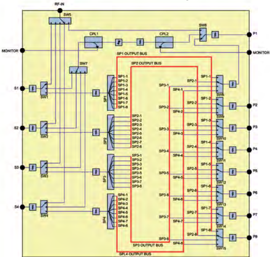
ZT-188 Functional Block Diagram
