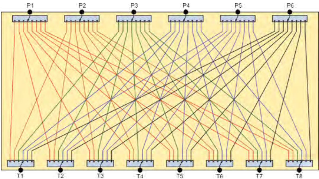
Functional Schematic of 6 x 8 Port RF Switch Matrix
