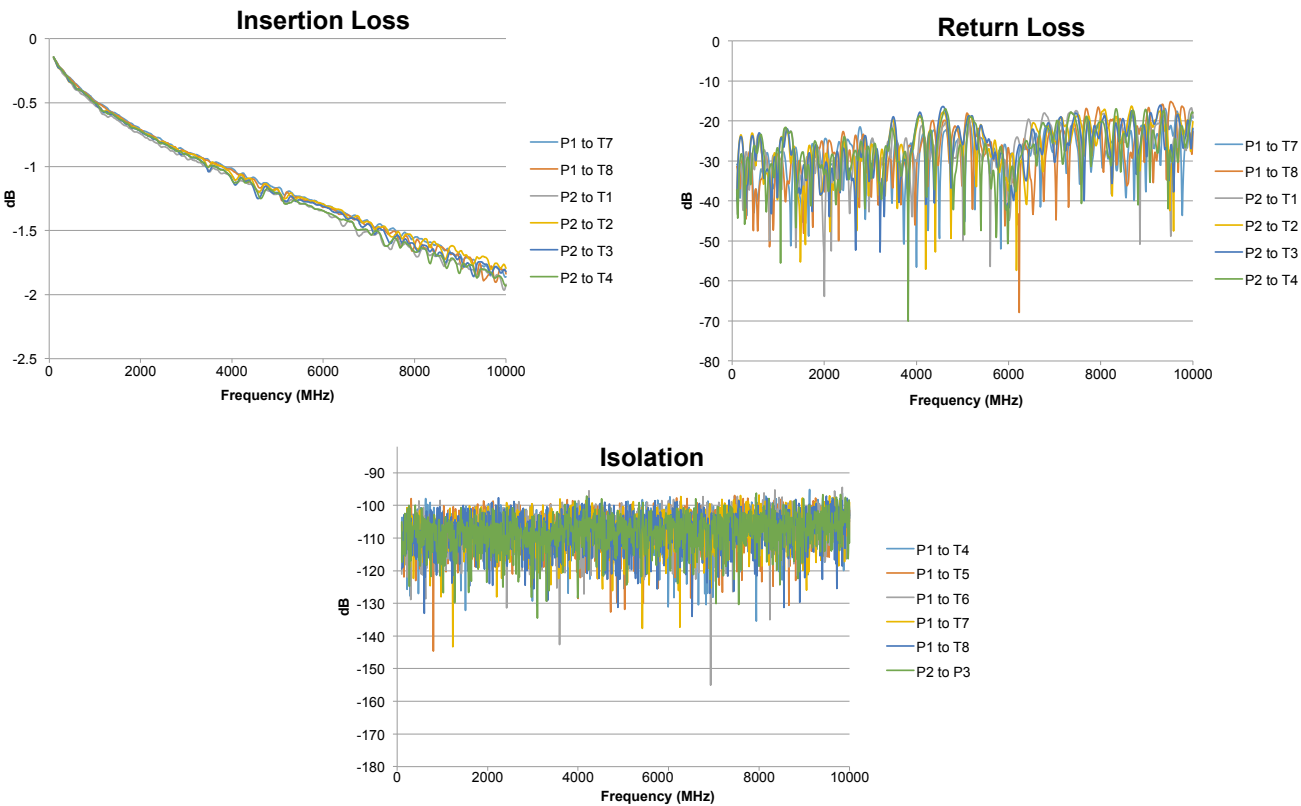
ZT-175 Curves
