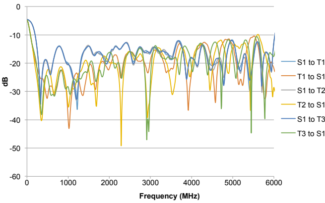
Typical Return Loss
