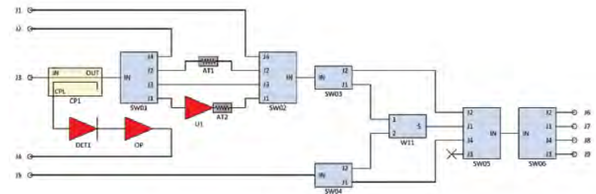
ZT-190A/B Functional Schematic
