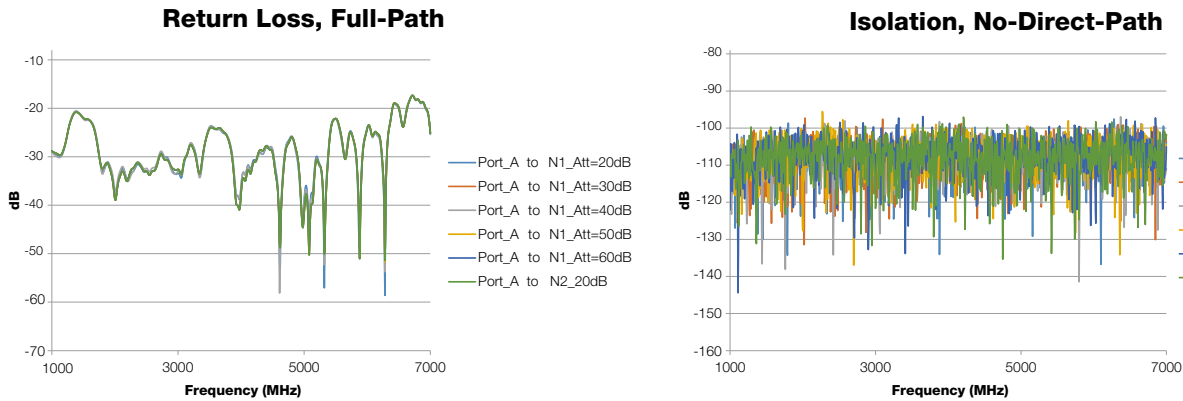
ZT-191 Curves
