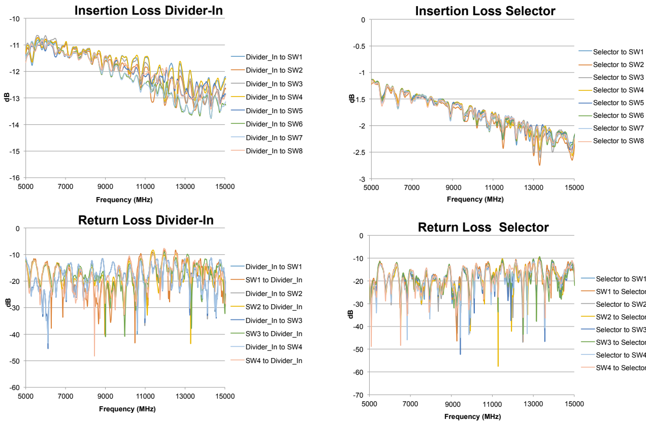
ZT-185 Curves
