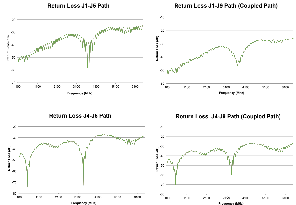
ZT-187 Curves
