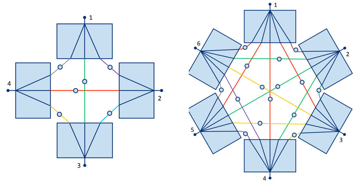
Common mesh network requirement, clockwise from top right: 4-port mesh; 6-port mesh; 9-port mesh
