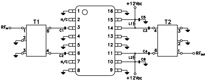
APPLICATION SCHEMATIC DIAGRAM (see table above for values C1 to C6, L1 & L2)
