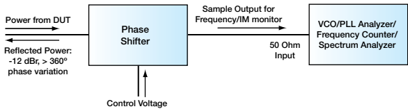
APPLICATION BLOCK DIAGRAM VCO (DUT) Load Pull Test
