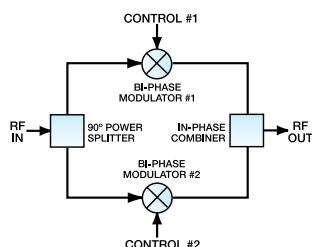
QPSK Block Diagram
