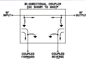
ELECTRICAL SCHEMATIC SYDC SERIES
