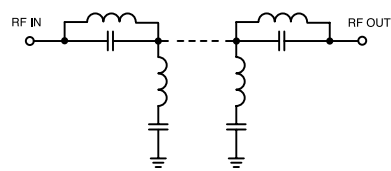
FUNCTIONAL SCHEMATIC
