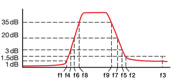
TYPICAL FREQUENCY RESPONSE
