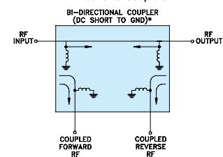
Bi-Directional Couplers
