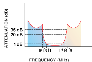
PBP Bandpass, Elliptical PBP-35N, PBP-35W
