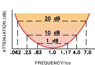
PIF Bandpass, Constant Impedance
