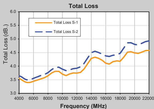
EP2K+ (5000-20000MHz)
