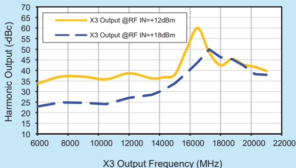
Harmonic X3 Output
