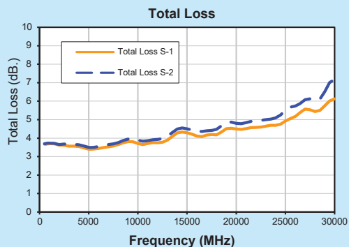
EP2K1+ (2000-26500MHz)
