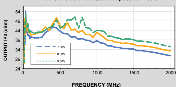
OUTPUT IP3 vs. FREQUENCY & DEVICE VOLTAGE INPUT POWER = 5.00dBm, Temperature = +25°C
