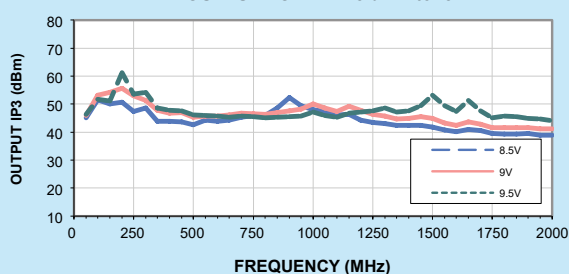
OUTPUT IP3 vs. FREQUENCY & DEVICE VOLTAGE OUTPUT POWER = 8 dBm/tone
